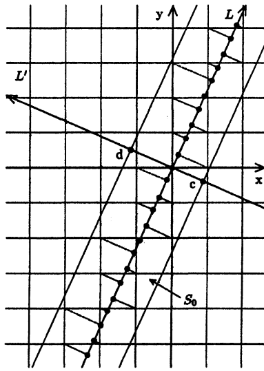
FIGURE 1. One-dimensional quasicrystal with \beta' < 0 .
